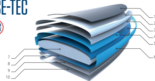
1- Deck Pad. / 2&10- Thermoformed plastic skin (ASA). / 3- 50g/m² Fiberglass wrap. 4&8- 200g/m² Woven Fiberglass. / 5- 200g/m² Woven Fiberglass Reinforcement Patch in standing area. / 6- 200g/m² Woven Fiberglass Rail Reinforcement. 7- Molded, Watertight EPS Foam Core. / 9- 50g/m² Fiberglass wrap.
