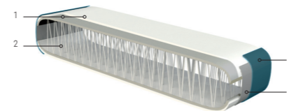
1- Fusion PVC double layer / 2- Nylon Drop-Stitch core 3- Outer PVC layer rail / 4- Inner PVC layer rail
