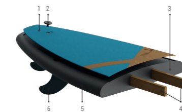
1- Brushed EVA deck PAD / 2- Leash plug 3- High density cellular foam / 4- Dual wooden Stringers 5- Textured surface / 6- Soft STELLAR fins
