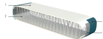
1- Single PVC layer / 2- Nylon Drop-Stitch core 3- Outer PVC layer rail / 4- Inner PVC layer rail
